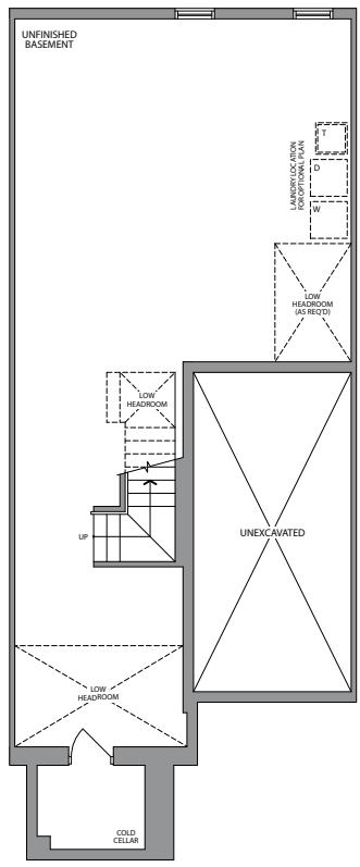
BASEMENT ELEVATION 1
