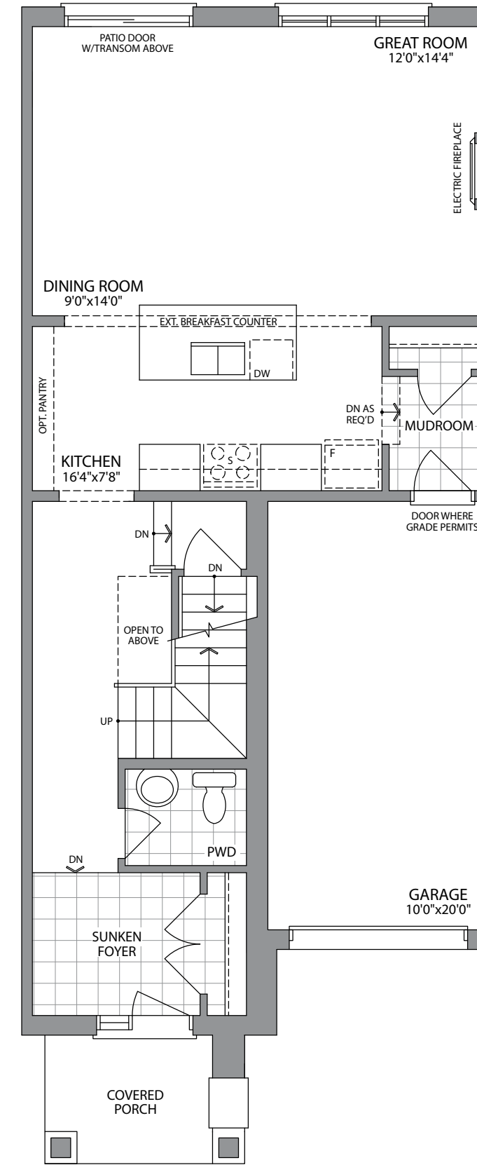
GROUND FLOOR ELEVATION 1
