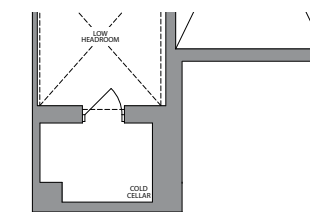
BASEMENT ELEVATION 2
