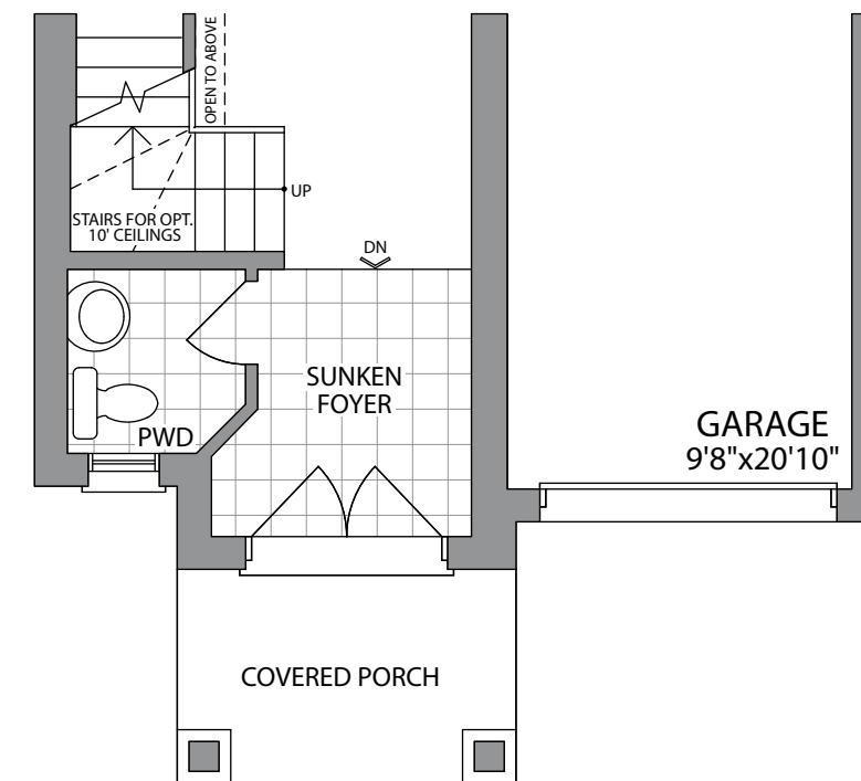
GROUND FLOOR ELEVATION 2
