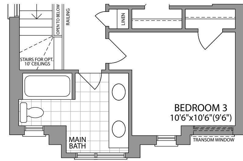
SECOND FLOOR ELEVATION 2
