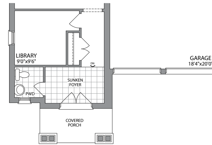
GROUND FLOOR ELEVATION 2
