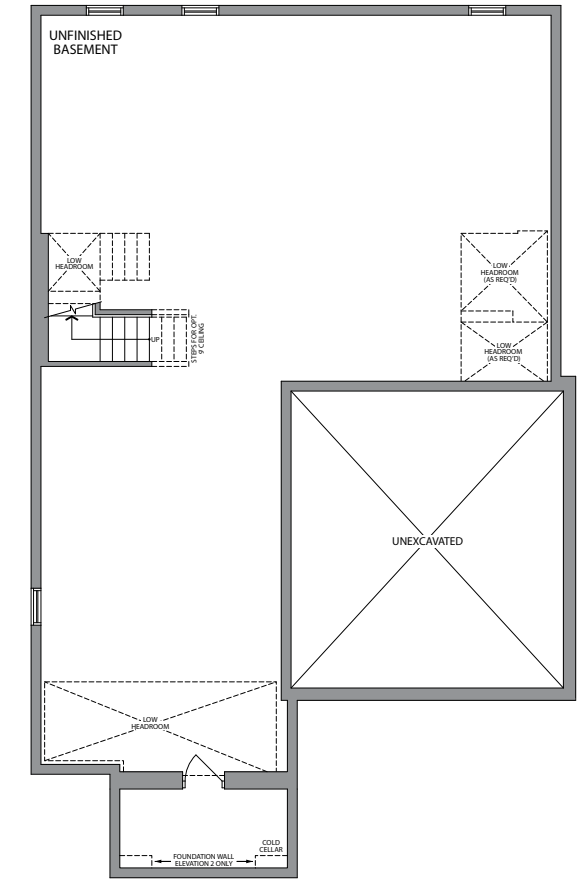
BASEMENT ELEVATION 1 & 2
