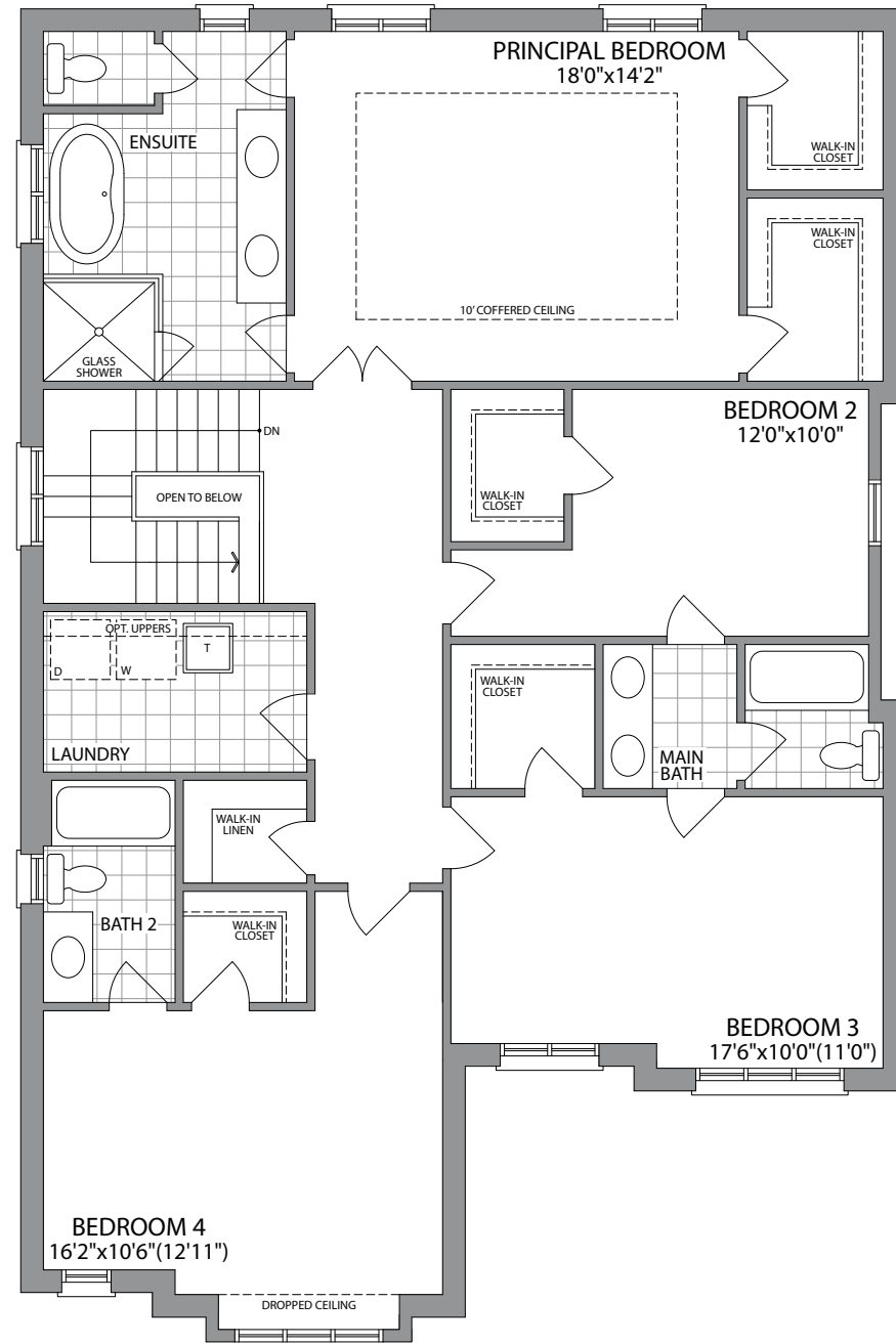
SECOND FLOOR ELEVATION 1
