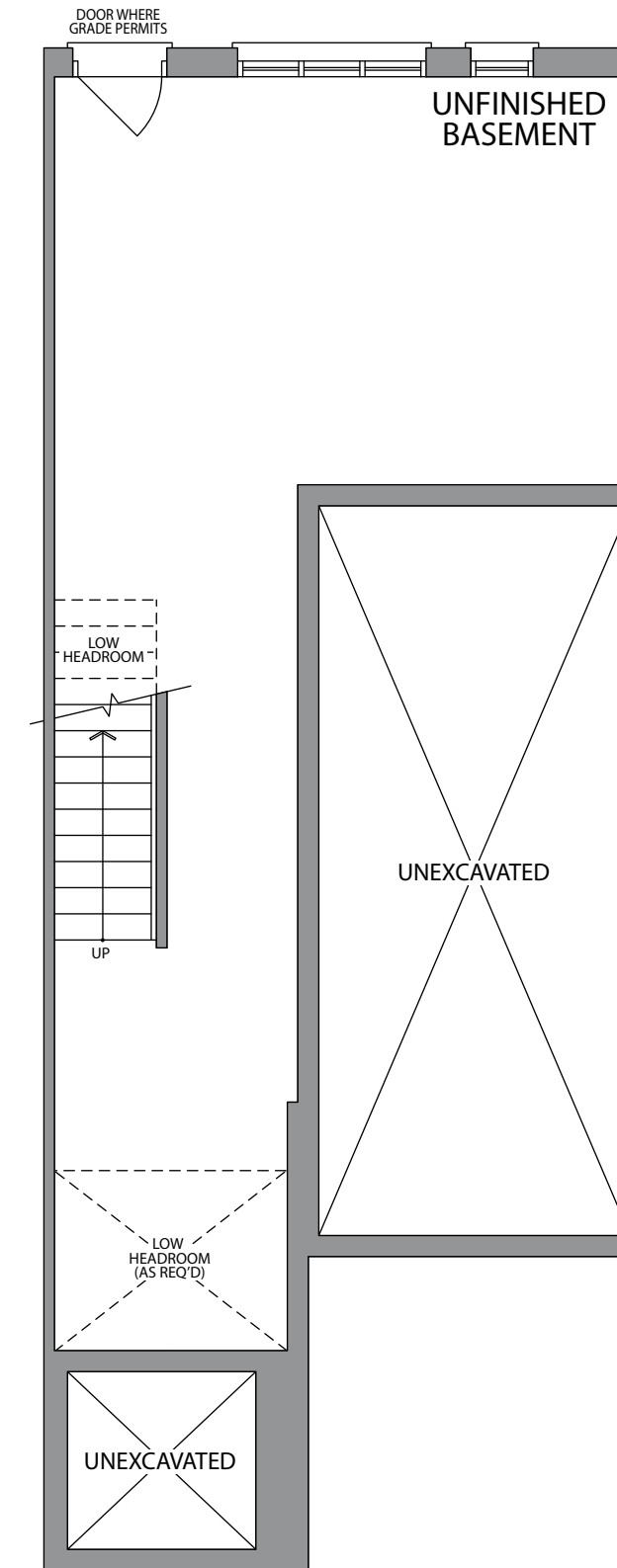
BASEMENT ELEVATION 1
